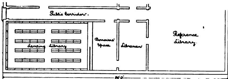
FIG. 18.—Lending Library arranged with Indicator for Fiction only (Section 125).
